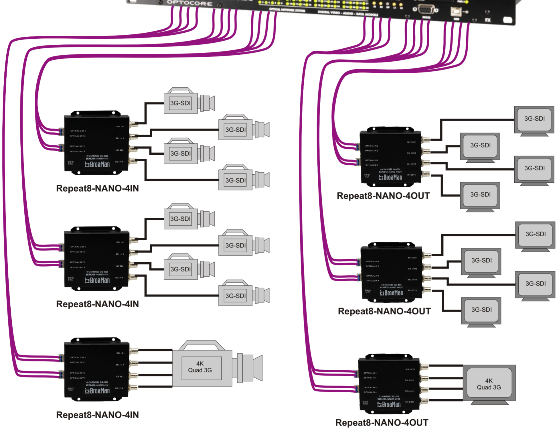
Route66 Video Router
